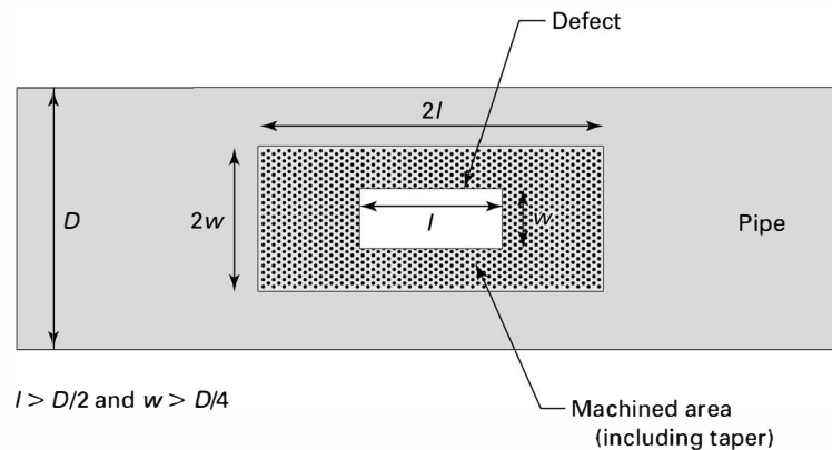
Figure 405-III-2-1 Defect Dimensions
