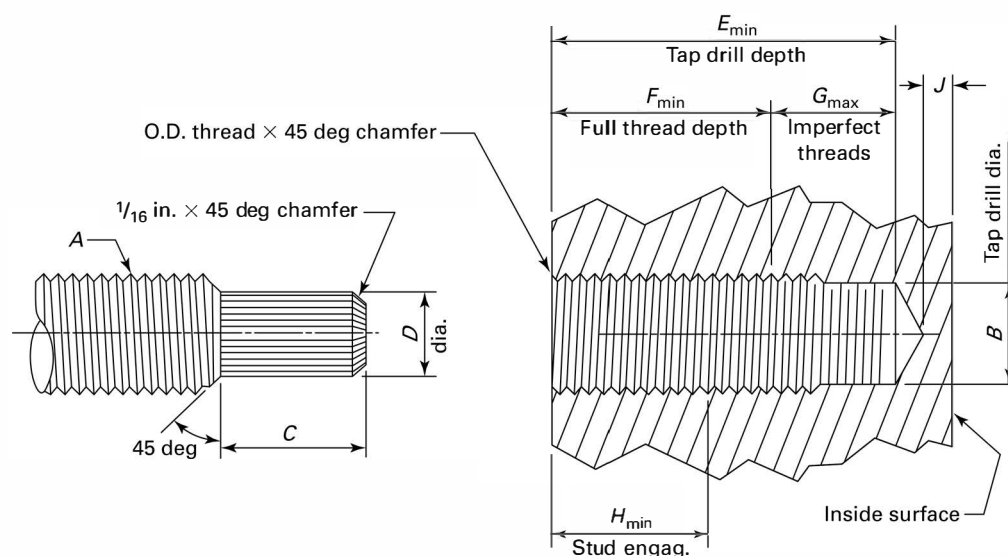
Figure 303-I-1 Inch Thread Series (U.S. Customary Units)
